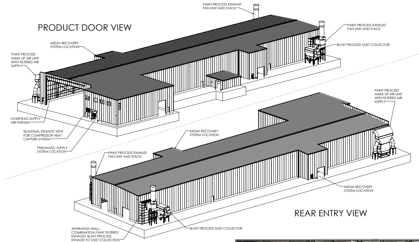
Proposal drawing of the all-in-one barge finishing facility
